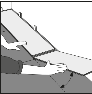
Step 5 Fit the second plank
