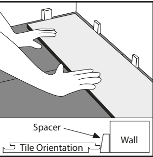
Step 4 Lay the first plank with tongue side facing wall using spacers
