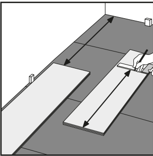
Step 6 Cut and fit the final plank in the first row
