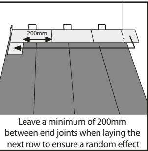
Step 7 (optional) Use offcut from previous row
