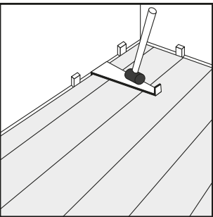
Step 10 Pullbar and rubber mallet can be used for the final row of planks, ensuring an expansion gap
