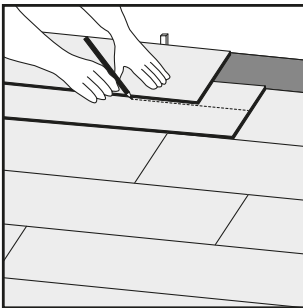
Step 9 Measure and cut the final row of planks, allowing for an expansion gap
